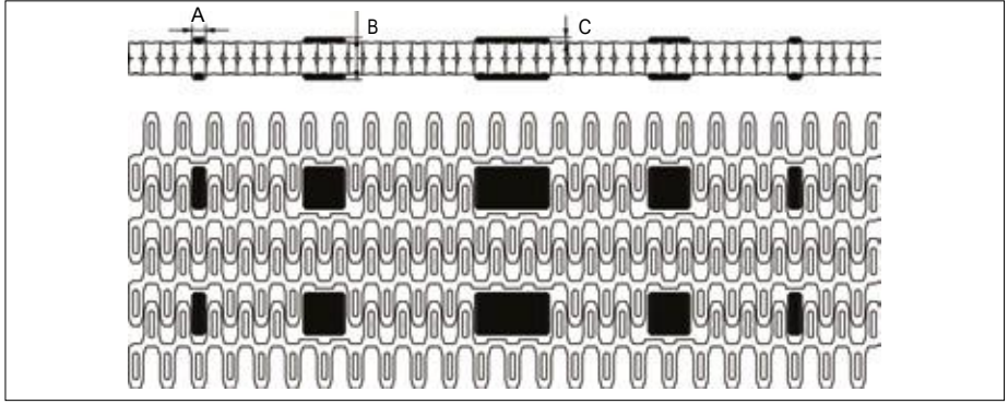
Made-To-Order Materials: POM-D, PP, PA6.6 and Roller Material POM-D. Non standard Roller material and color: See uni Material and Color overview.
