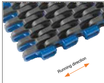
uni Flex SNB CI Rubber Top R2.3 Surface Opening: 47%
